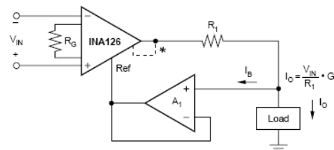
Fig. 2 Voltage to current converter circuit
