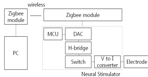
Fig. 1 System configuration block
