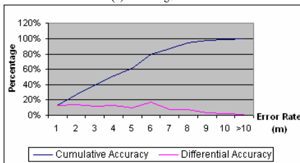
(b) TN Algorithm
