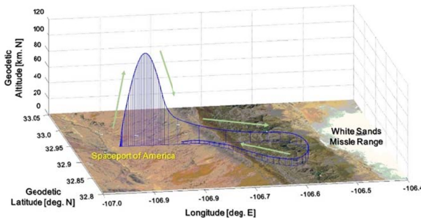
Fig. 4 Flight profile of WIRES-X
