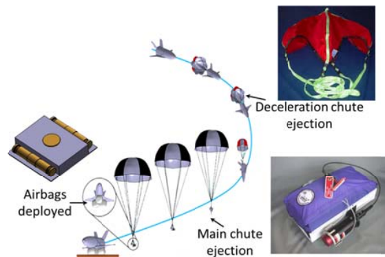
Fig. 32 Recovery systems
