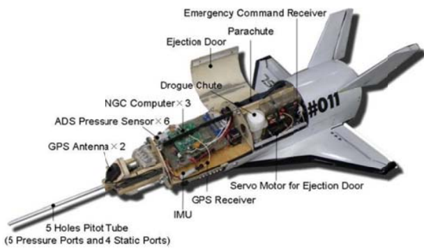
Fig. 6 Subsystem layout of WIRES#011
