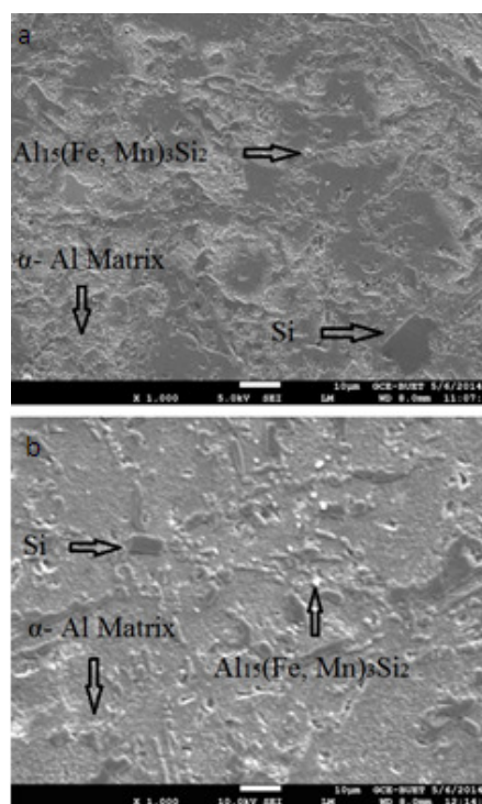
Fig. 7 SEM micrographs of as-received Al-Si (a) block and (b) piston
