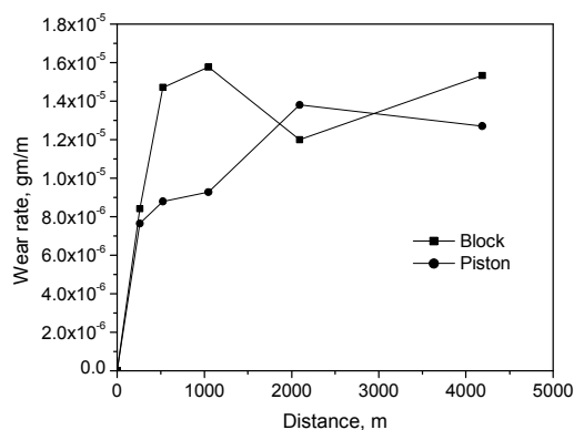
Fig. 4 Variation of wear rate (gm/m) with the variation of sliding distance (m) at applied pressure of 1.4 MPa (Load 20N) and sliding velocity 0.29 \text{ ms}^{-1}
