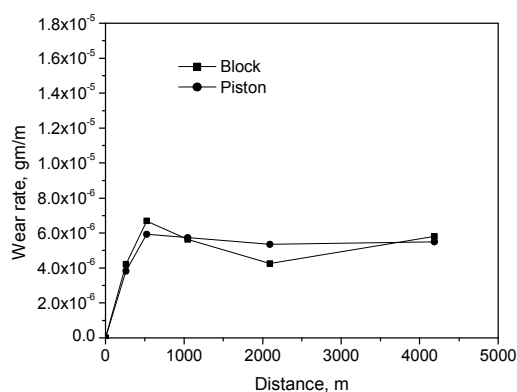
Fig. 3 Variation of wear rate (gm/m) with the variation of sliding distance (m) at applied pressure of 0.30 MPa (Load 5N) and sliding velocity 0.29 \text{ ms}^{-1}
