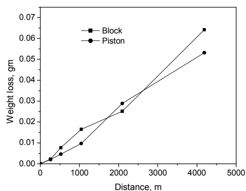
Fig. 2 Variation of weight loss (gm) with the variation of sliding distance (m) at applied pressure of 1.4 MPa (Load 20N) and sliding velocity 0.29 \text{ ms}^{-1}
