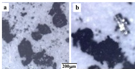
Fig. 6 Wear debris collected from wear test at 1.4 MPa (20N) applied pressure and sliding distance of 4200m for (a) Block, (b) Piston
