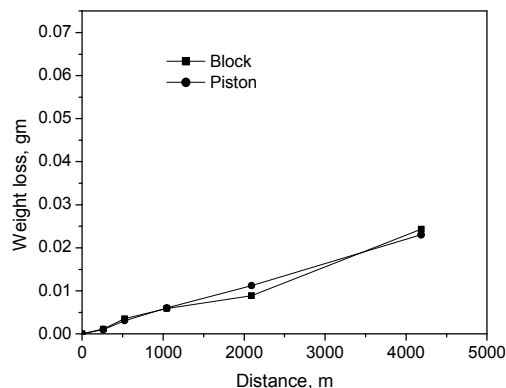
Fig. 1 Variation of weight loss (gm) with the variation of sliding distance (m) at applied pressure of 0.30MPa (Load 5N) and sliding velocity 0.29 \text{ ms}^{-1}
