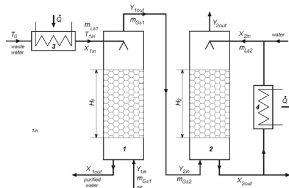
Fig 1 Scheme of the process
