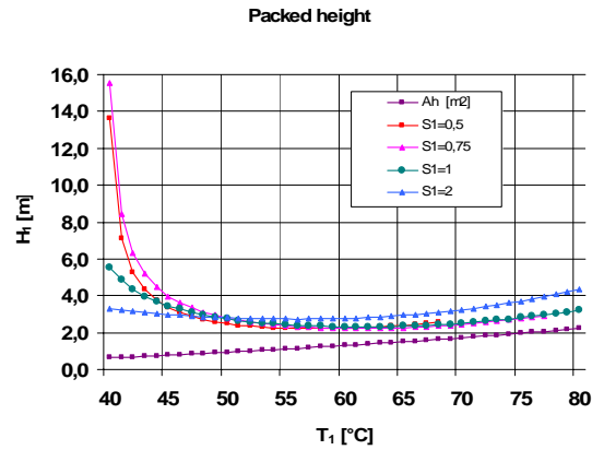
Fig. 6 Packed height of the desorber column in function of temperature
