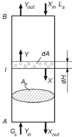
Fig. 2 Scheme of the absorber and desorber column
