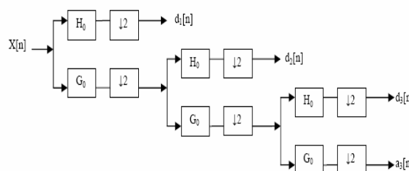
Fig. 7 Three-level wavelet decomposition tree
