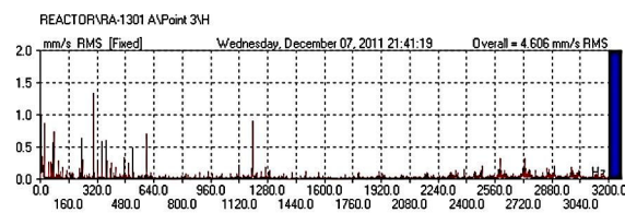
Fig. 10 FFT in close monitoring condition
