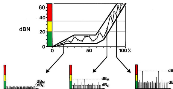
Fig. 3 Steps in measuring SPM
