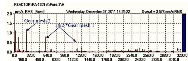
Fig. 8 Vibration data (FFT) in couple condition start up
