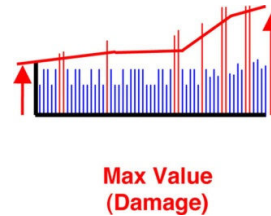
Fig. 5 Maximum Value (Bearing or gear Damage)
