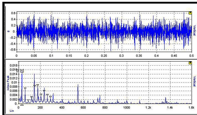
Fig. 1 FFT and TWF samples in GMF
