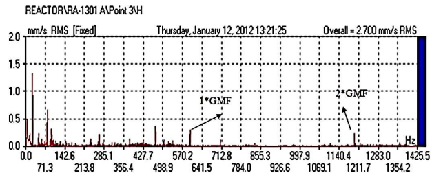
Fig. 15 FFT in critical point in horizontal direction
