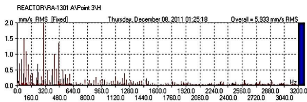
Fig. 11 FFT after 12 hours close monitoring
