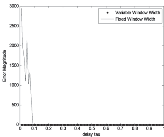
Fig. 7 Error of both receivers for \text{BOC}(10, 5)
