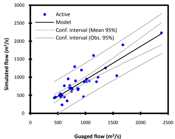
Fig. 4 Simulated versus observed monthly flow during the calibration period (1990-1992)
