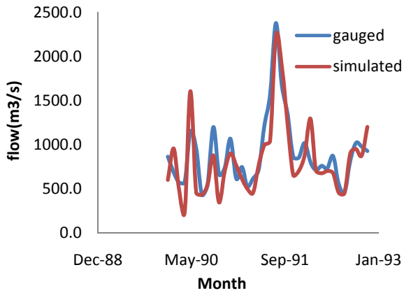
Fig. 5 Simulated and Observed flows during the calibration period (1990-1992)
