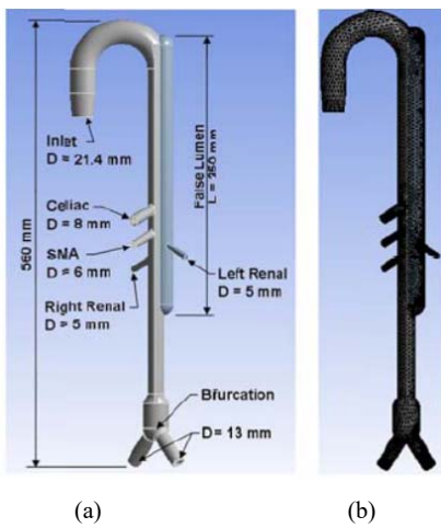
Fig. 1 (a) Schematic diagram of the dissection model, (b) Mesh
