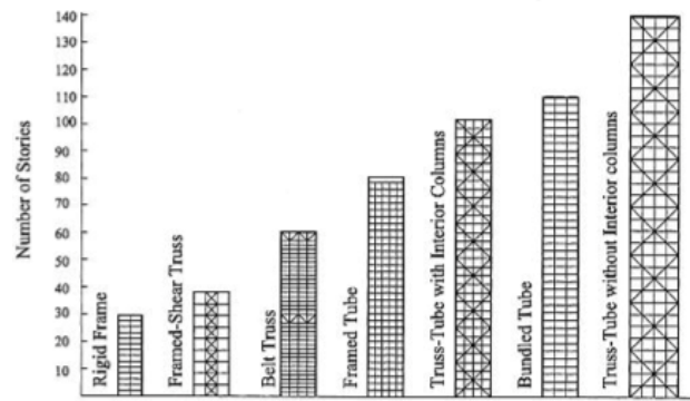
Fig. 2 Classification of steel tall buildings structure [21], [23]
