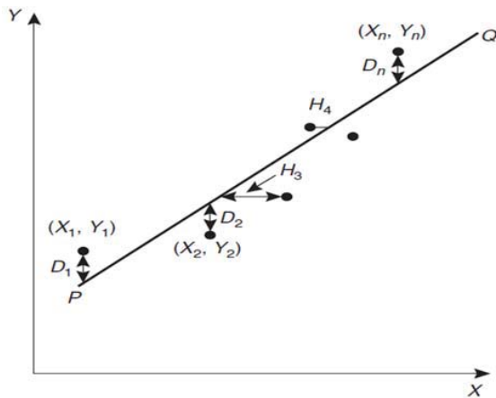
Fig. 2 The least-squares regression lines
