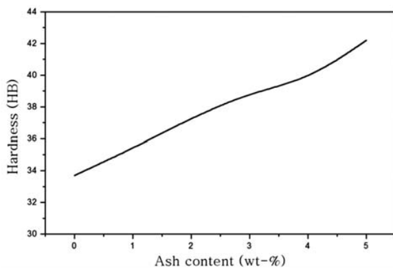
Fig. 4 Hardness change with ash content
