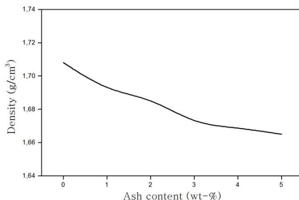
Fig. 2 Density vs ash content
