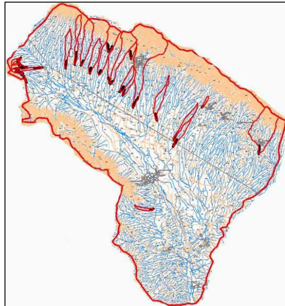
Fig. 4 position map of gullies and their basin areas
