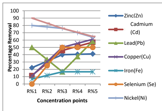
Fig. 1 Heavy Metal % Removal at pH 7.8
