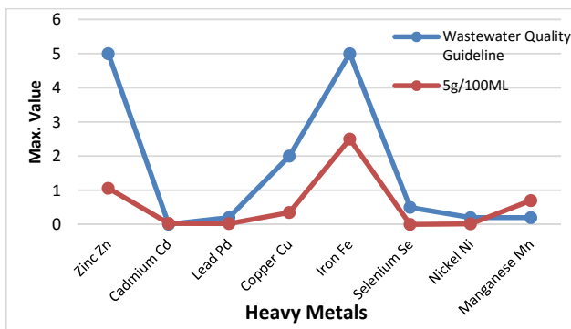
Fig. 4 Experimental Results and Quality Guidelines at pH 7.8
