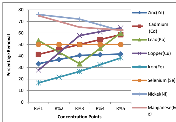
Fig. 2 Heavy metal % removal at pH 6.8
