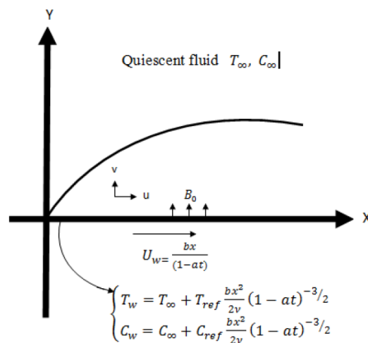
Fig. 1 Physical flow model
