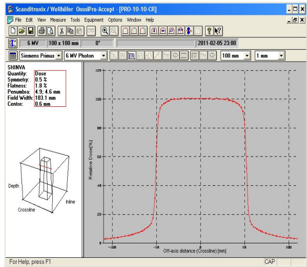
Fig. 3 Standard Field (10*10) Measurement With semiconductor
