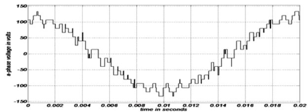
Fig. 9.b A-phase phase voltage with over-modulation.
