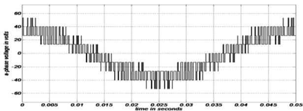
Fig. 7.c A-phase phase voltage with f_1=20\text{Hz} .
