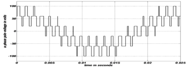
Fig. 8.a A-phase pole-voltage with f_1=40\text{Hz} .
