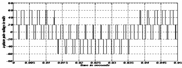
Fig. 7.a A-phase pole-voltage with f_1=20\text{Hz} .
