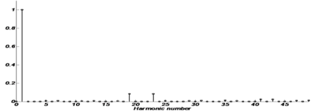
Fig. 9.c Normalized harmonic spectrum of the phase voltage with over-modulation
