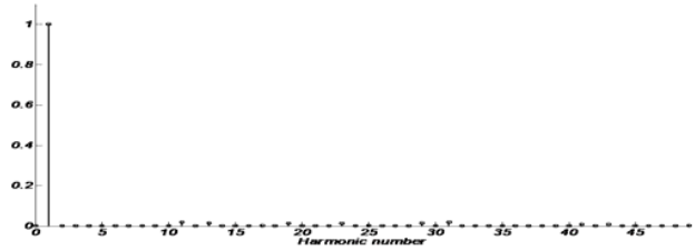
Fig. 8.c Normalized harmonic spectrum of the phase voltage with f_1=40\text{Hz} .
