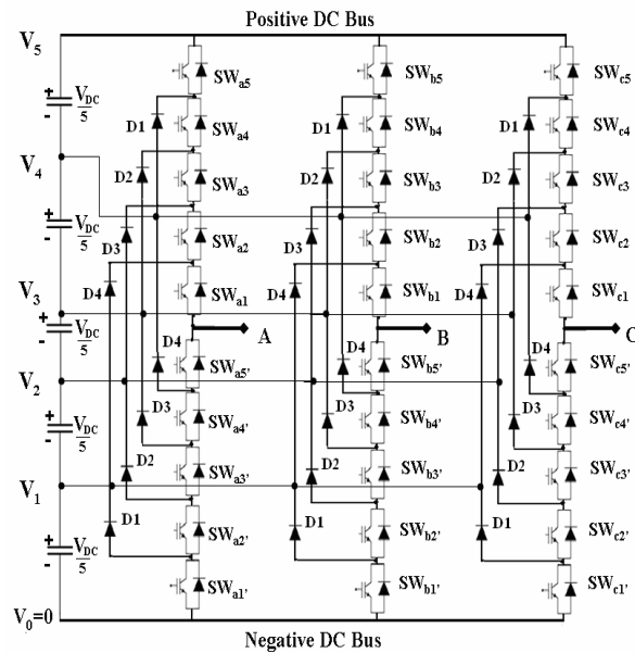
Fig. 1 Schematic of the six-level diode-clamped inverter configuration
