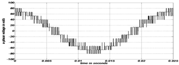
Fig. 8.b A-phase phase voltage with f_1=40\text{Hz} .
