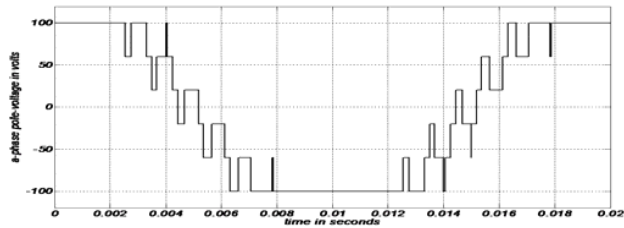
Fig. 9.a A-phase pole-voltage with over-modulation.
