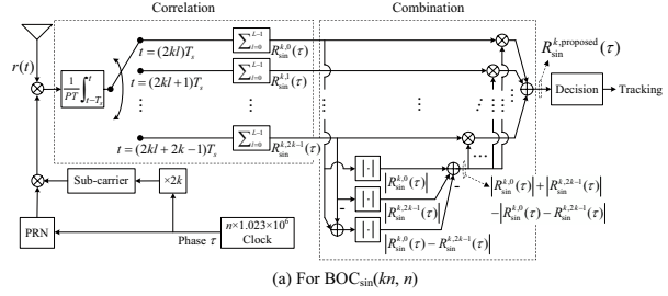
(a) For \text{BOC}_{\sin}(kn, n)
