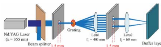
Fig. 1 Schematic of two-beam laser interference patterning
