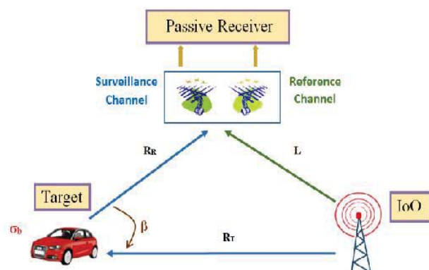
Fig. 1 Basic PBR geometry
