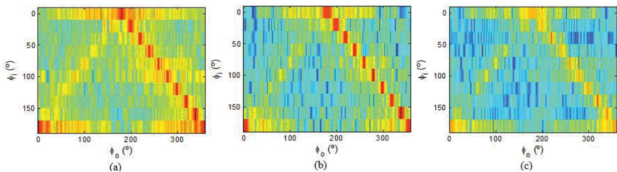
Fig. 4 2D BRCS maps for three representative vehicle models: (a) Audi5, (b) Mazda 6 sport and (c) Peugeot 307
