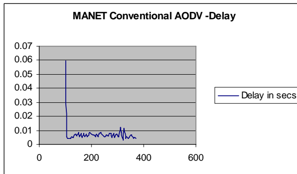
Fig. 1 AODV Delay
