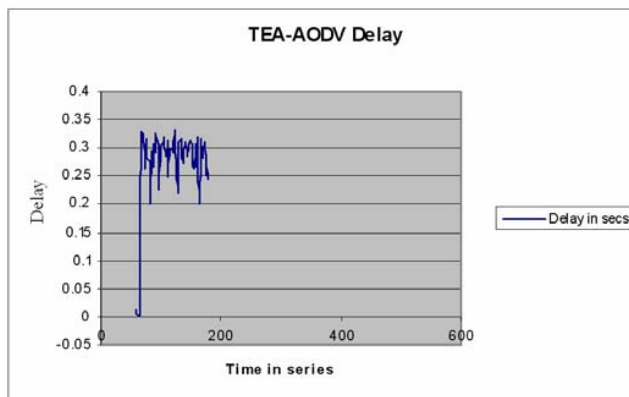
Fig. 2 TEA-AODV Delay
