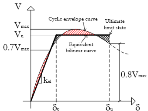
Fig. 22 Bilinear Idealization
