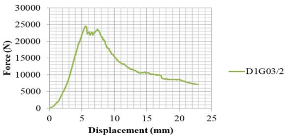
Fig. 13 Force-displacement diagram of the D1G03-2
