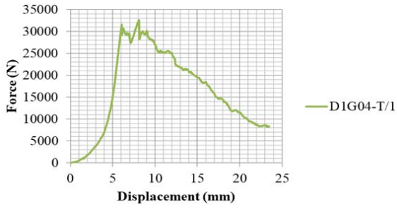
Fig. 17 Force-displacement diagram of the D1G04-T/1
