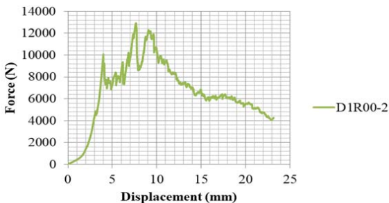
Fig. 7 Force-displacement diagram of the D1R00-2
