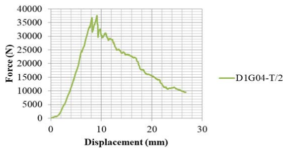
Fig. 19 Force-displacement diagram of the D1G04-T/2
