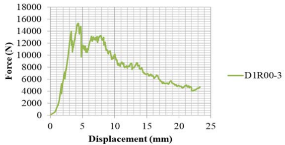
Fig. 9 Force-displacement diagram of the D1R00-3
