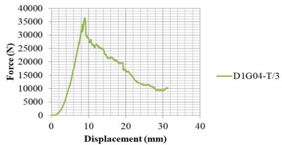
Fig. 21 Force-displacement diagram of the D1G04-T/3
