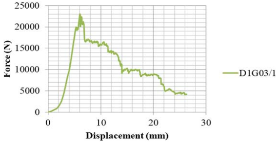
Fig. 11 Force-displacement diagram of the D1G03-1
