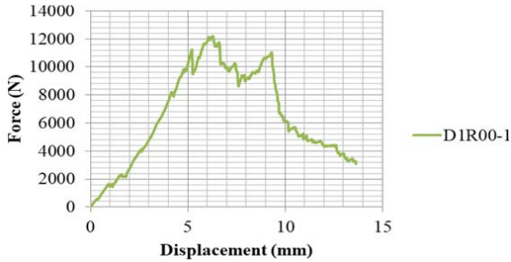
Fig. 5 Force-displacement diagram of the D1R00-1
