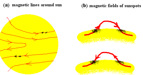
Fig. 7 (a) Magnetic field structure around the sun (b) structure of magnetic lines that form the sunspots
