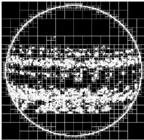
Fig. 9 Quad tree decomposition of sunspot trajectories of September 2001
