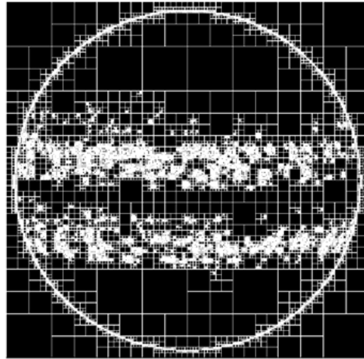
Fig. 10 Quad Tree decomposition of sunspot trajectories of October 2001
