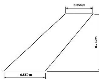
Fig. 5 Geometric configuration of AGARD 445.6 wing
