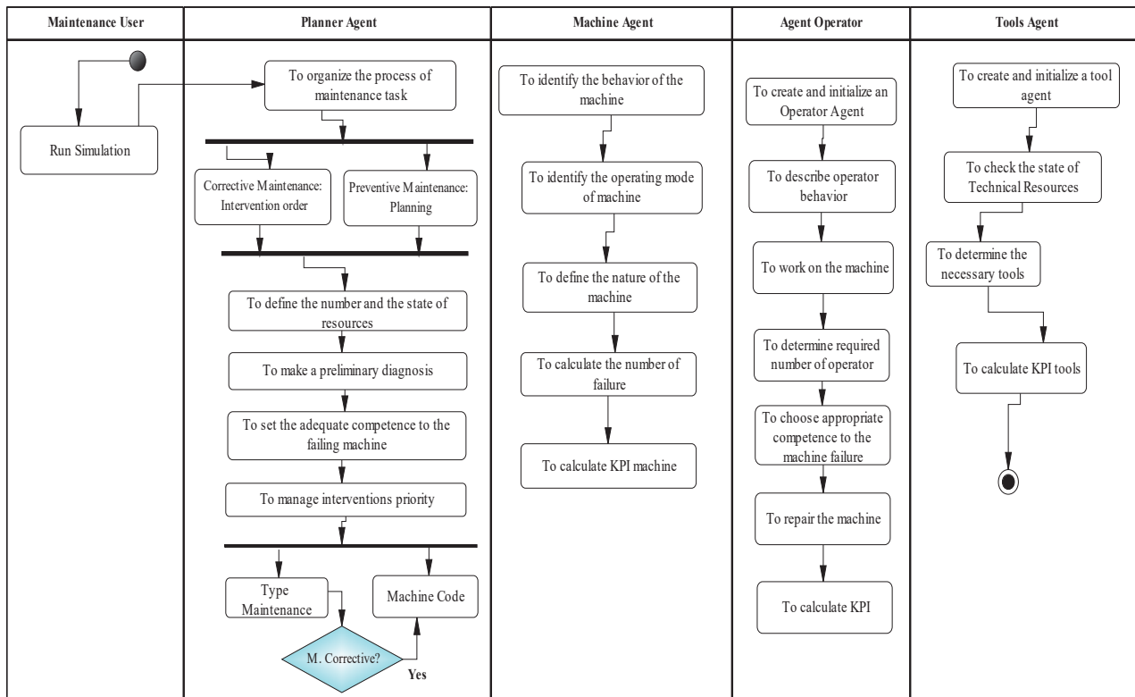
Fig. 2 Activity diagram of Agents
