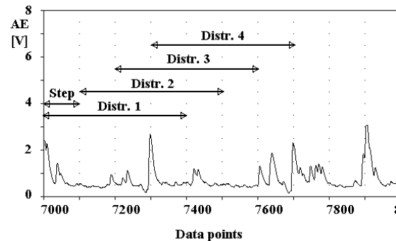
Fig. 4 Overlapping distributions
