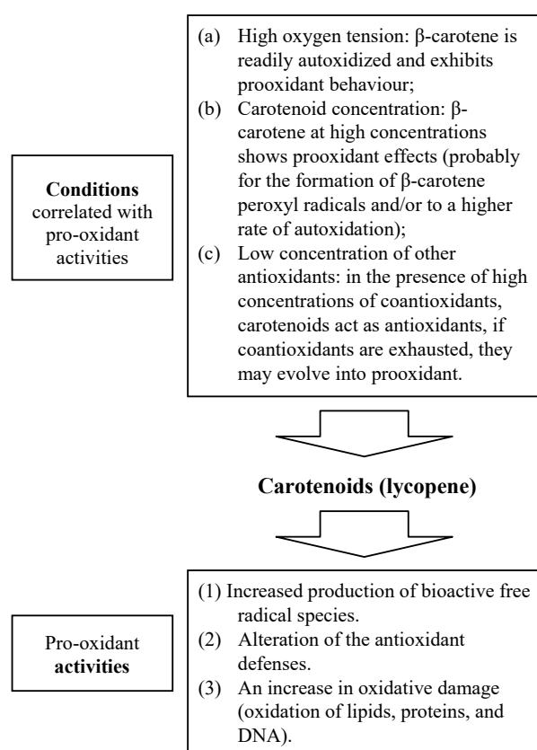
Fig. 3 Prooxidant activity of carotenoids (lycopene) [104]
