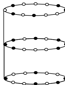
Fig. 5 PSO optimized thinned array (47.22% filling)
