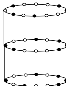
Fig. 7 PSO optimized thinned array (47.22% filling)
