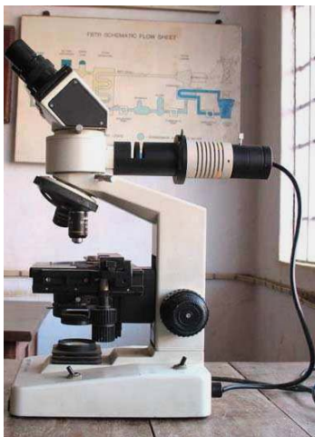
Fig. 7 Metallurgical Microscope
