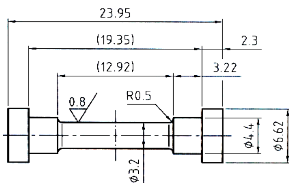
Fig. 3 Tensile Test Specimen
