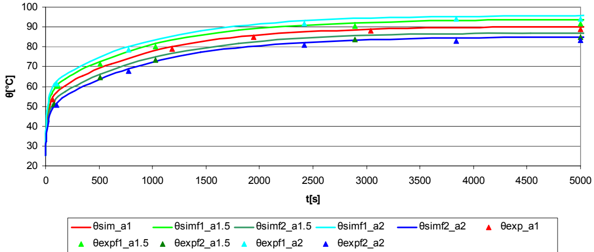
Fig. 9 Maximum fuse links temperature time evolution for current value of 160A and different asymmetry coefficient a = 1, 1.5, 2 . Comparison between simulation ( \theta_{\text{sim}}_{a1}, \theta_{\text{sim}}_{a1.5}, \theta_{\text{sim}}_{a2}, \theta_{\text{sim}}_{a1.5}, \theta_{\text{sim}}_{a2} ) and experimental values ( \theta_{\text{exp}}_{a1}, \theta_{\text{exp}}_{a1.5}, \theta_{\text{exp}}_{a2}, \theta_{\text{exp}}_{a1.5}, \theta_{\text{exp}}_{a2} )
