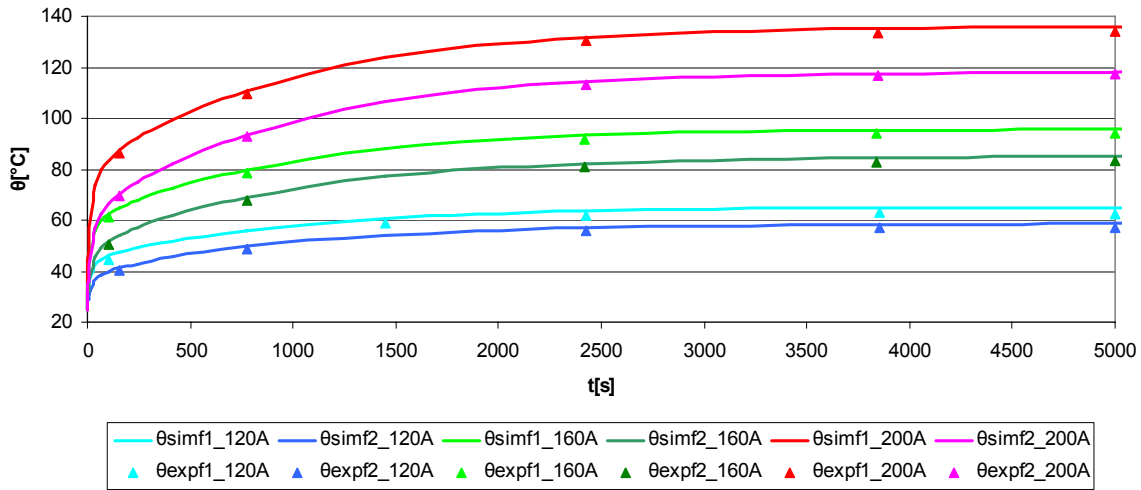
Fig. 10 Maximum fuse links temperature time evolution for current value of 120, 160 and 200A with the asymmetry coefficient a = 2 . Comparison between simulation ( \theta_{\text{sim}}_{120A}, \theta_{\text{sim}}_{160A}, \theta_{\text{sim}}_{200A}, \theta_{\text{sim}}_{120A}, \theta_{\text{sim}}_{160A}, \theta_{\text{sim}}_{200A} ) and experimental values ( \theta_{\text{exp}}_{120A}, \theta_{\text{exp}}_{160A}, \theta_{\text{exp}}_{200A}, \theta_{\text{exp}}_{120A}, \theta_{\text{exp}}_{160A}, \theta_{\text{exp}}_{200A} )
