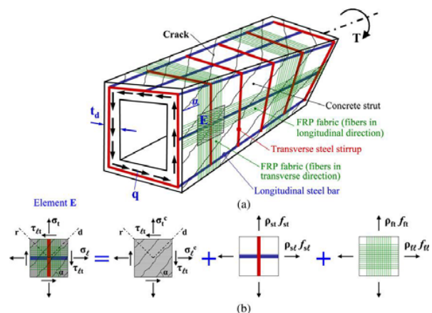
Fig. 1 Space truss for the torsional analysis of R.C. beam strengthened with FRP composites [6]
