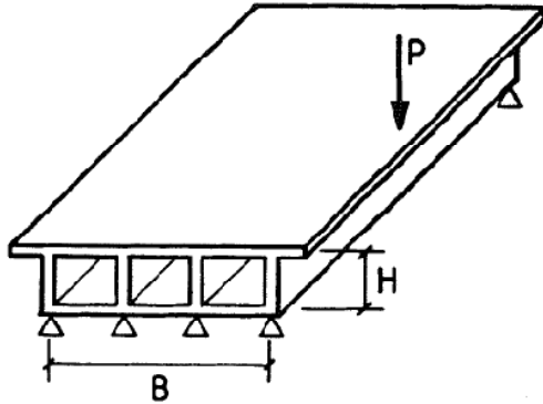
Fig. 2 Multi-cell box girder under torsion [21]
