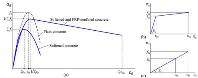
Fig. 3 Constitutive stress–strain laws for the materials: (a): concrete; (b): steel; (c): FRP [6]
