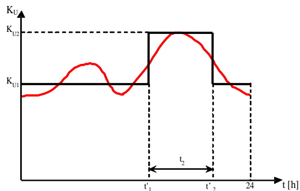
Fig. 2 Approximation of the daily load curve
