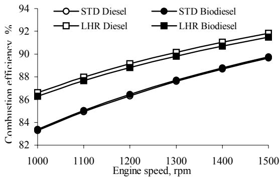
Fig. 19 Variation of combustion efficiency at full load
