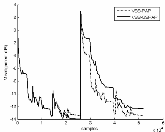
Fig. 5. Misalignments of VSS-PAP and VSS-GSPAP. Single-talk case, L=512 , under-modelling scenario, SNR=30 dB, echo path change after 26000 samples.
