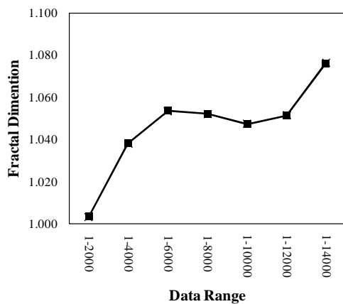
Fig. 3 Fractal dimension of Ghareh-Aghaj River daily time series in different selection windows by R/S Method
