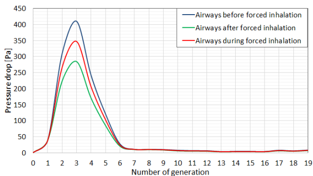
Fig. 10 Pressure drop in the airways during forced inhalation
