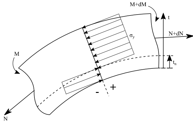
Fig. 14 Stress distribution during plastic deformation
