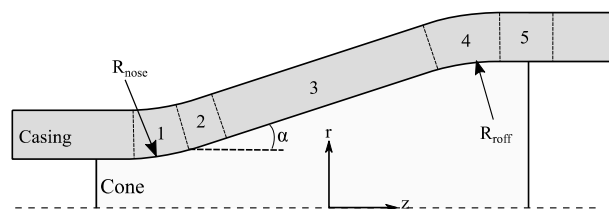
Fig. 3 Stages of plastic deformation of casing during expansion. A: cone, B: Expandable casing. (1) bending outward, (2) bending inward, (3) diameter increase (4) bending inward (5) bending outward
