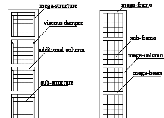
Fig. 2 MSCSS configuration
