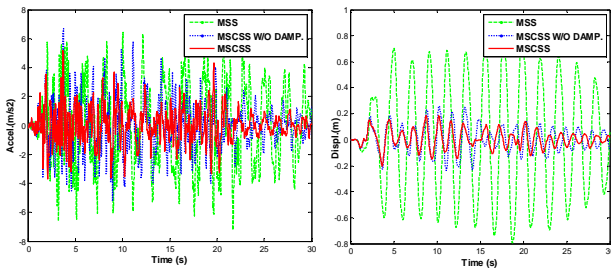
Fig. 5 mega-frame top floor acceleration and displacement under El Centro wave (0.4g)
