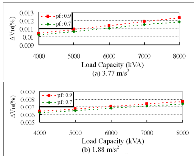
Fig. 12 The voltage flicker curve of two wind generators with in reactive power control mode, under average wind speed variance ratios of 3.77 and 1.88 \text{ m/s}^2 , corresponding to various capacity and load power factors
