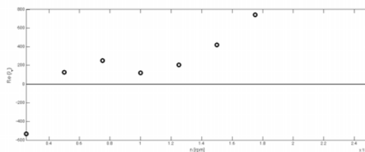
Fig. 11. Dependency of real parts of eigenvalues on rotating speed for damped system.
