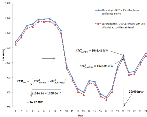
Fig. 2 ATC and TRM variations considering uncertainty of transmission line outages on 1 st March 2002
