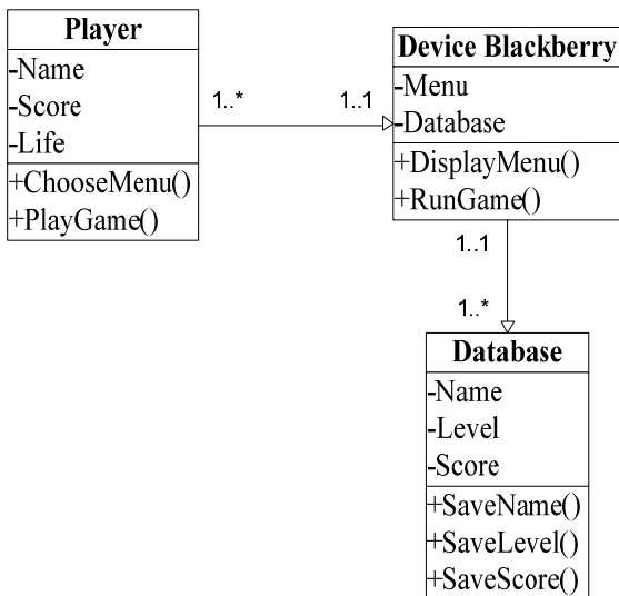
Fig. 3 Class diagram of the adaptive games
