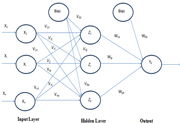
Fig. 1 Neural network with 3 inputs and 1 output
