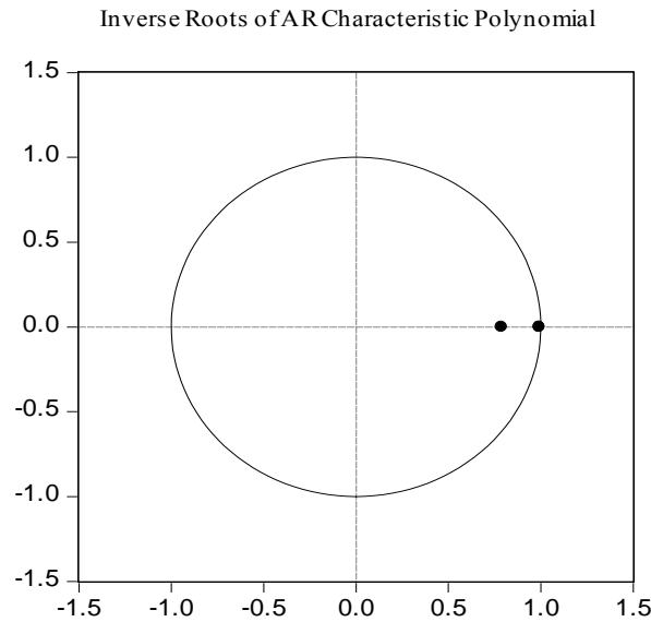
Fig. 2 Stationarity of the VAR (1) Model
