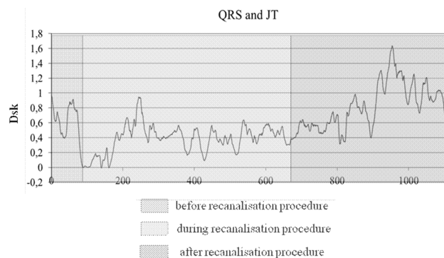
Fig. 7 Dynamical changes of interactions of ECG parameters
