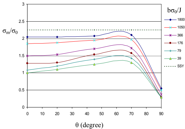
Fig. 6 Mean stress at r\sigma_0/J=2 as a function of the parametric angle \theta along the crack front at different levels of deformation for a semi-circular surface crack ( a/w=0.5, a/c=1 ) in tension.
