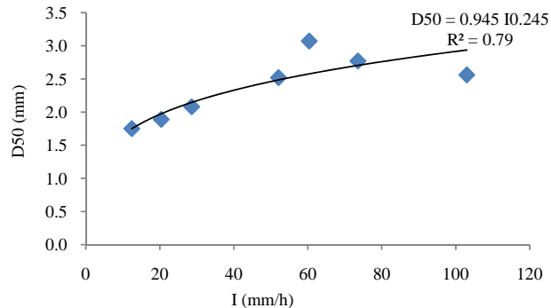
Fig. 1 Relationship between rainfall intensity and raindrop diameter
