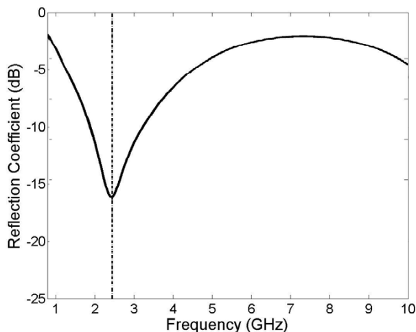
Fig. 6 The simulated reflection coefficient of the Unchoked antenna, expressed logarithmically. The dashed line represents the commonly used MWA frequency of 2.45 GHz
