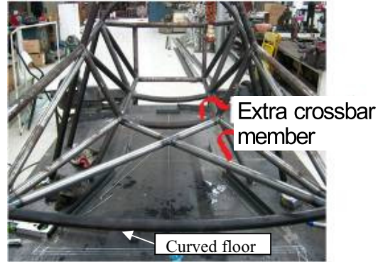
Fig. 15 Extra crossbar member
