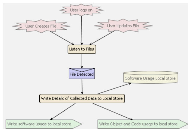
Fig. 8 Agent Overview Diagram for the Monitoring Agent
