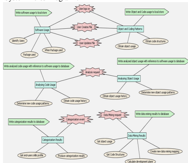
Fig. 3 System Roles Diagram
