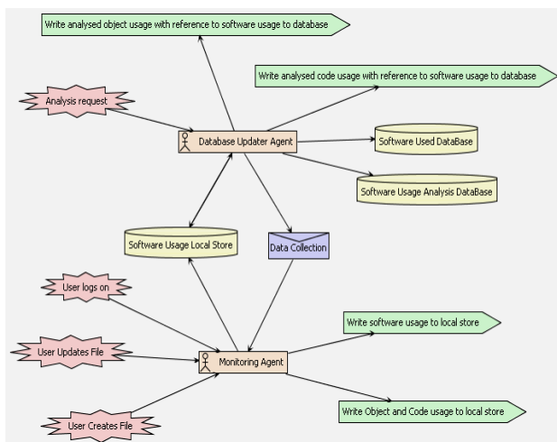
Fig. 7 System Overview Diagram
