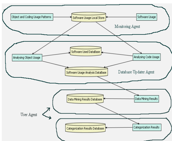
Fig. 4 Data Coupling Diagram
