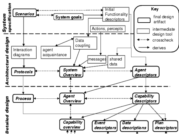
Fig. 1 The phases of Prometheus methodology
